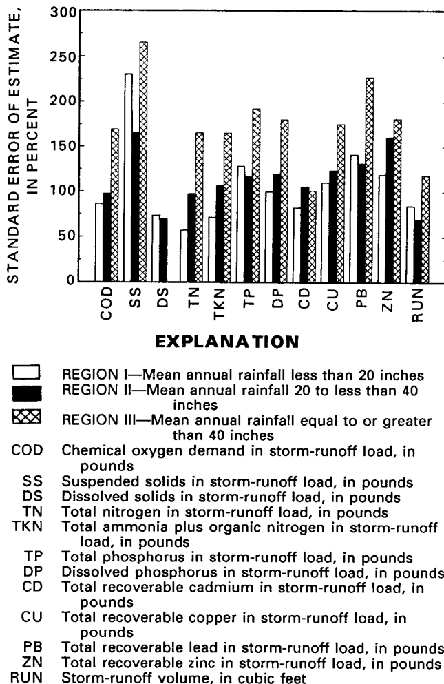
Figure 2. Standard errors of estimate for regression models of water-quality constituents and total runoff in three mean annual rainfall regions.
