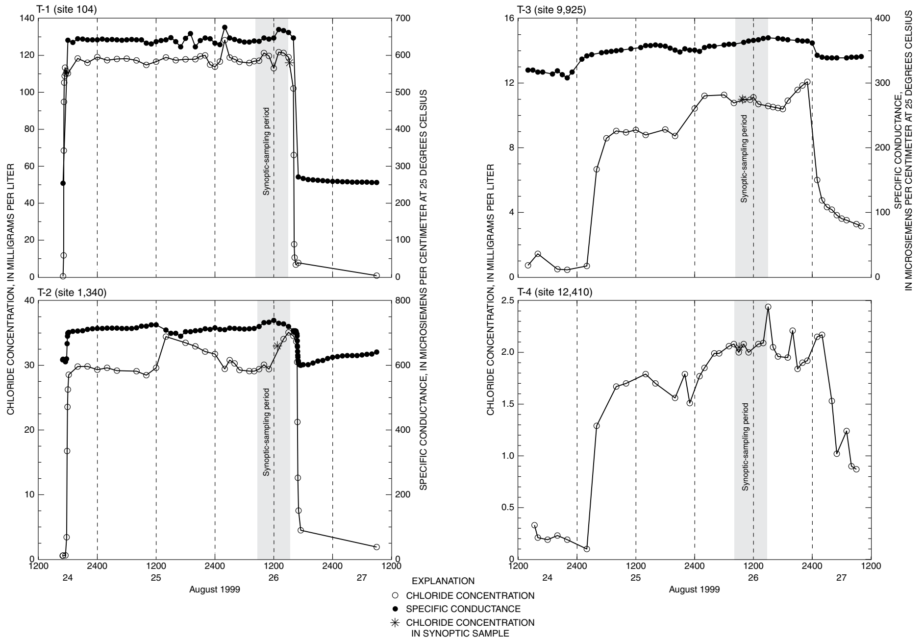
Figure 5. Temporal profiles of chloride concentration and specific conductance at tracer-monitoring sites on Daisy Creek and the Stillwater River, Montana, August 24-27, 1999. Temporal specific-conductance data were not collected at site T-4.
