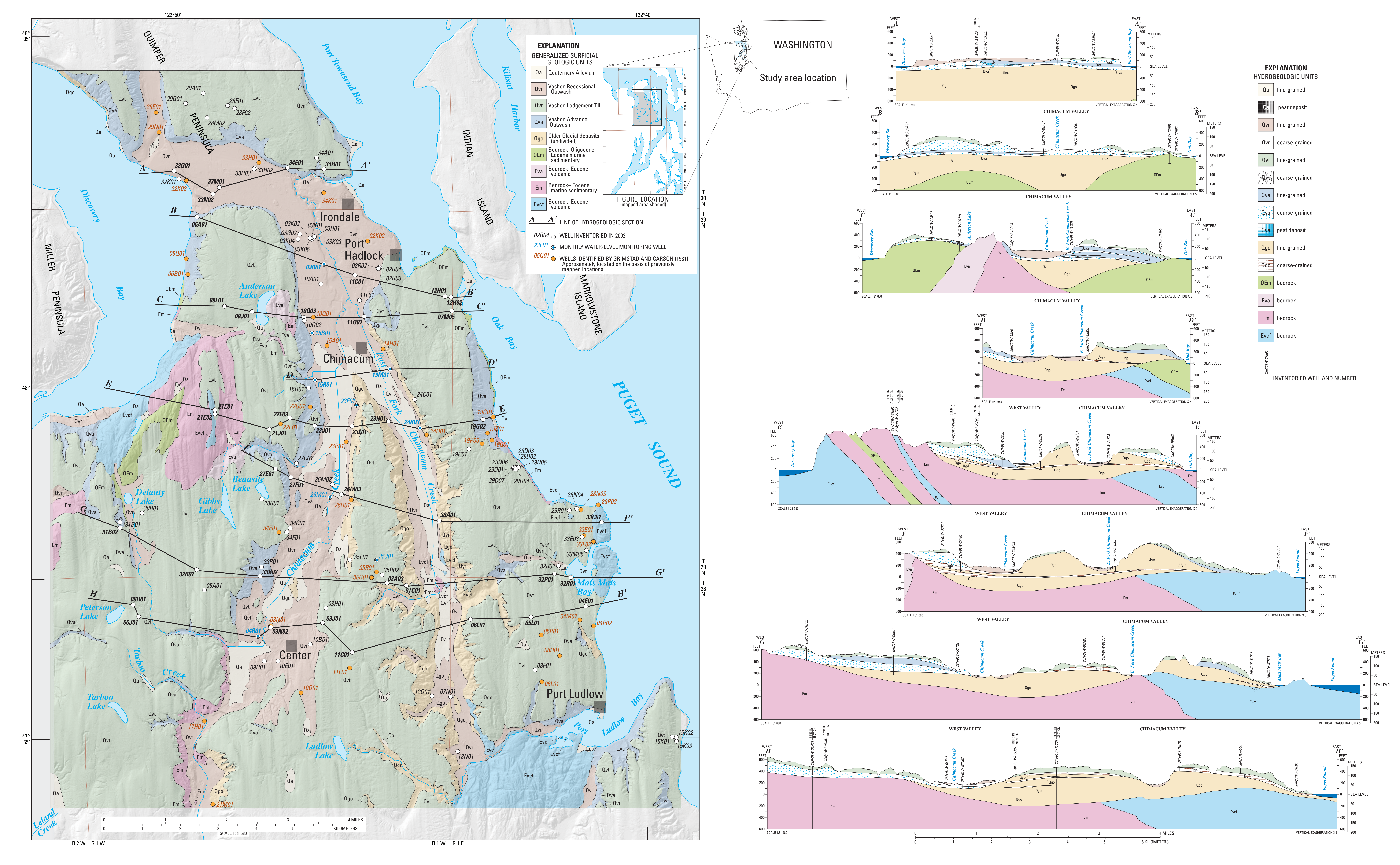
MAP SHOWING SURFICIAL GEOLOGY AND LOCATIONS OF INVENTORIED WELLS AND HYDROGEOLOGIC SECTIONS IN THE CHUMACUM CREEK BASIN, EASTERN JEFFERSON COUNTY, WASHINGTON
