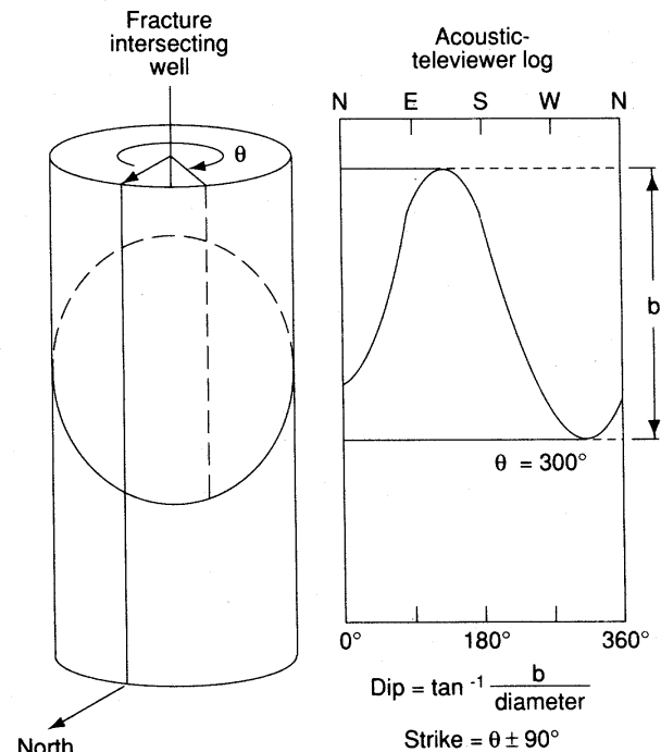
Figure 2. Fracture intersecting a well and corresponding acoustic-televiwer log and determination of strike and dip (modified from Paillet, 1985).
