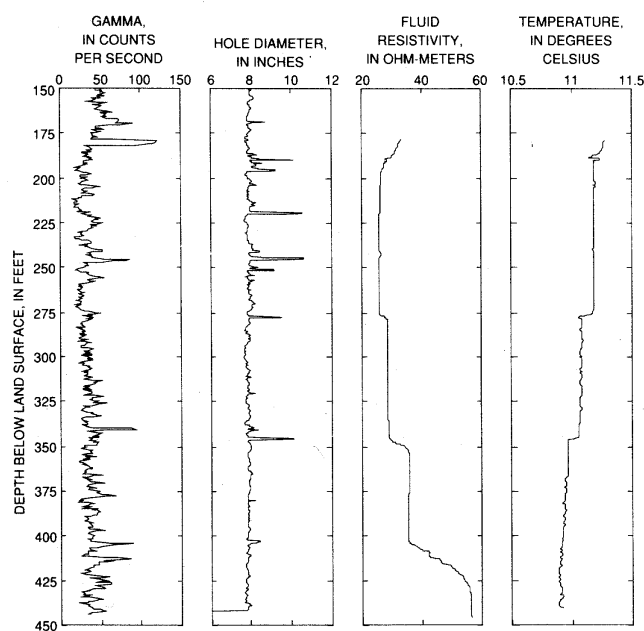
Figure 3. Gamma, caliper, fluid-resistivity, and temperature logs of well Ro82 at Spring Valley.
