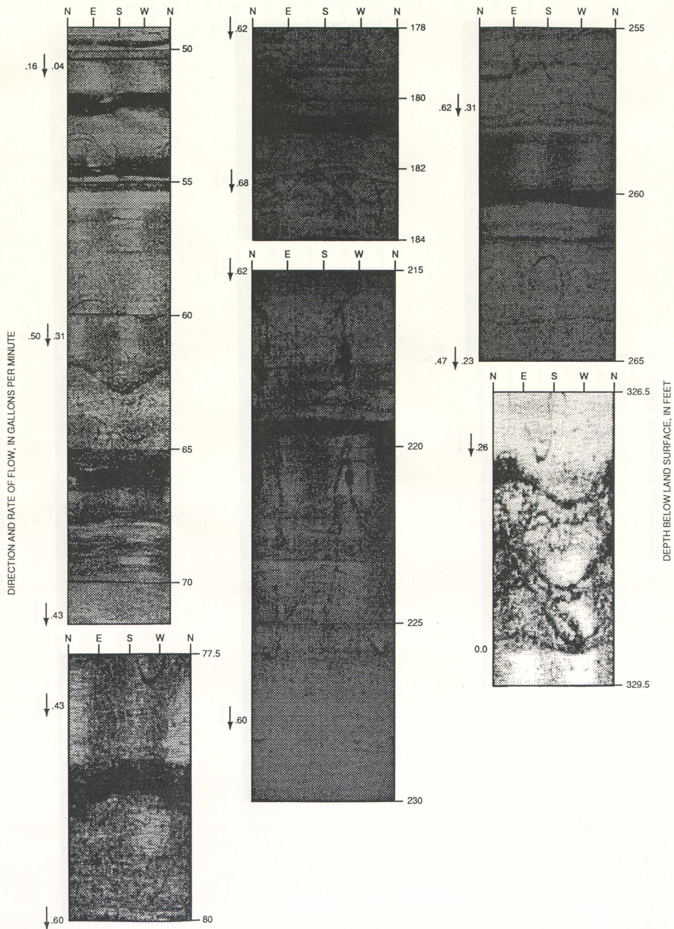
Figure 7. Acoustic-televiometer log of fracture zones and vertical-flow direction and rate as measured with the heat-pulse flowmeter in well P899 at Mahopac.
