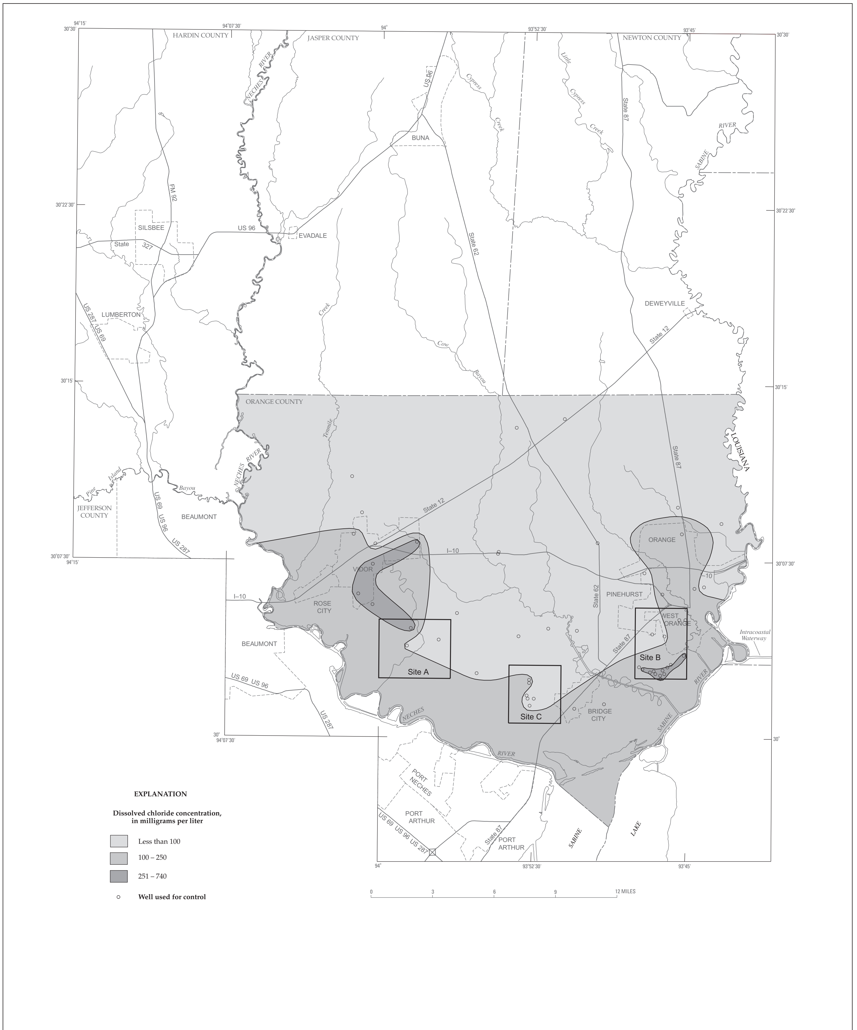
MAP SHOWING DISTRIBUTION OF DISSOLVED CHLORIDE CONCENTRATIONS IN WATER FROM WELLS SCREENED IN THE LOWER UNIT OF THE CHICOT AQUIFER IN ORANGE COUNTY, TEXAS, NOVEMBER-DECEMBER 1989
