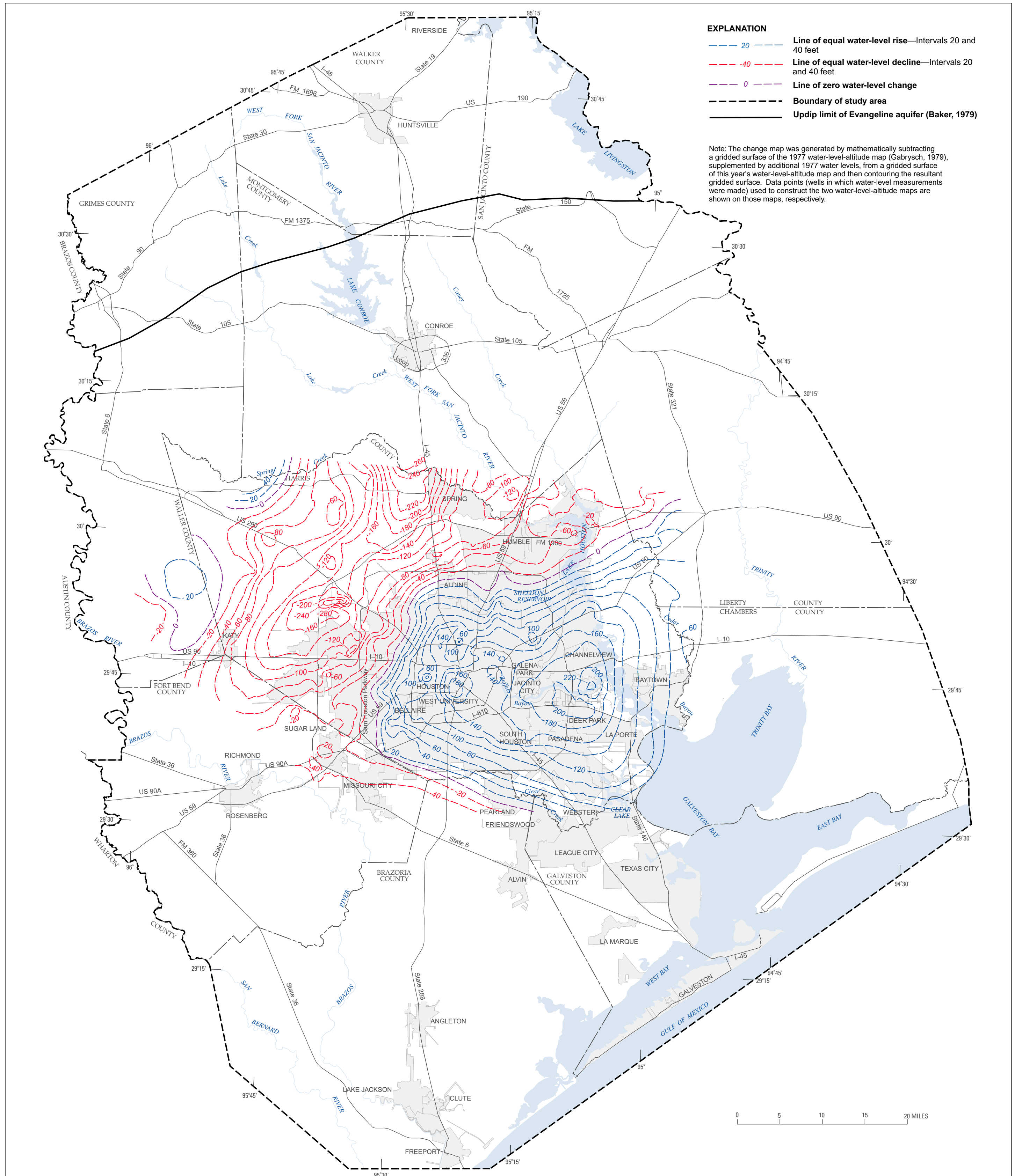
Figure 7. Map showing approximate water-level changes in the Evangeline aquifer, Houston-Galveston region, Texas, 1977-2004.
