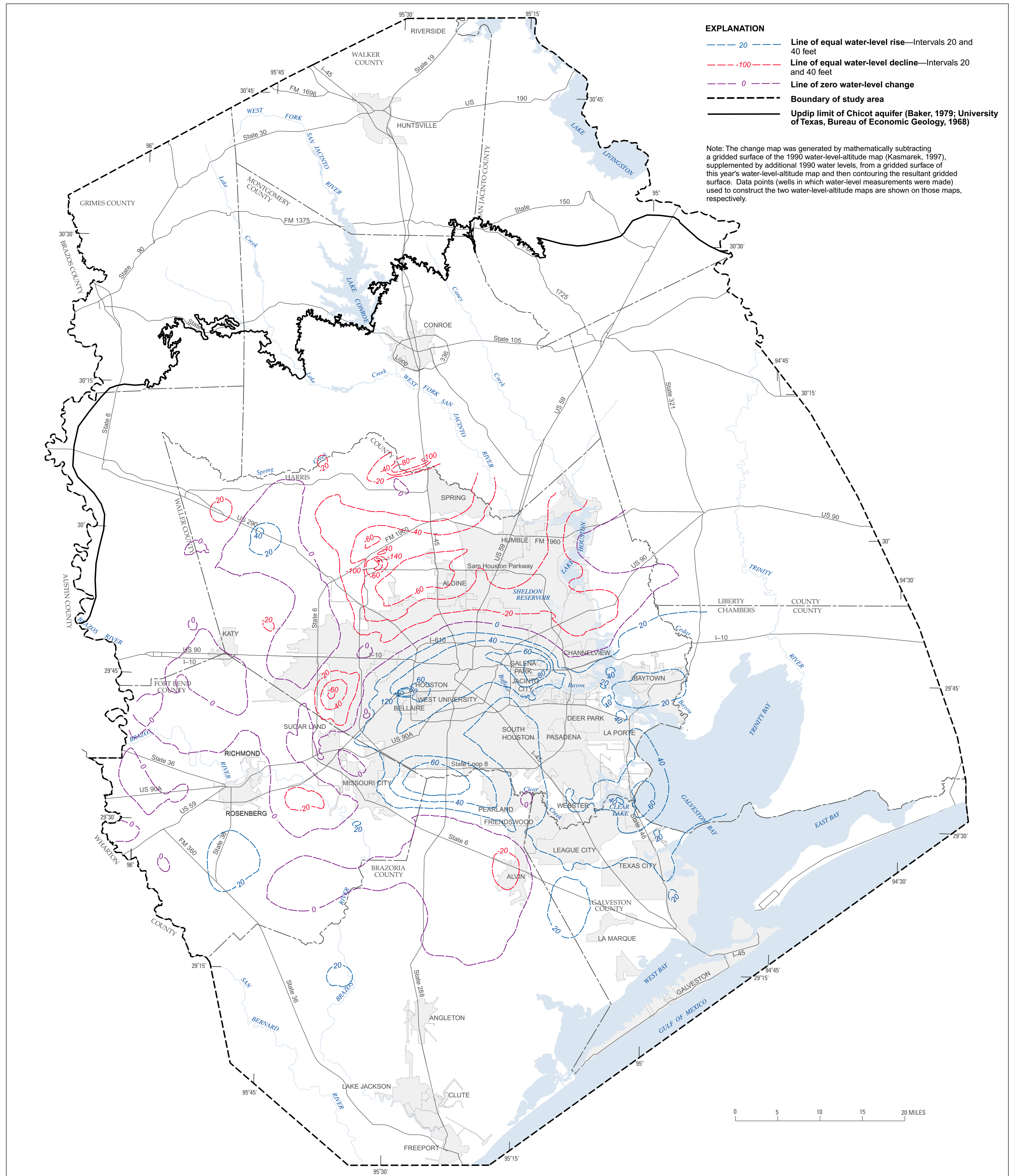
Figure 4. Map showing approximate water-level changes in the Chicot aquifer, Houston-Galveston region, Texas, 1990-2004.
