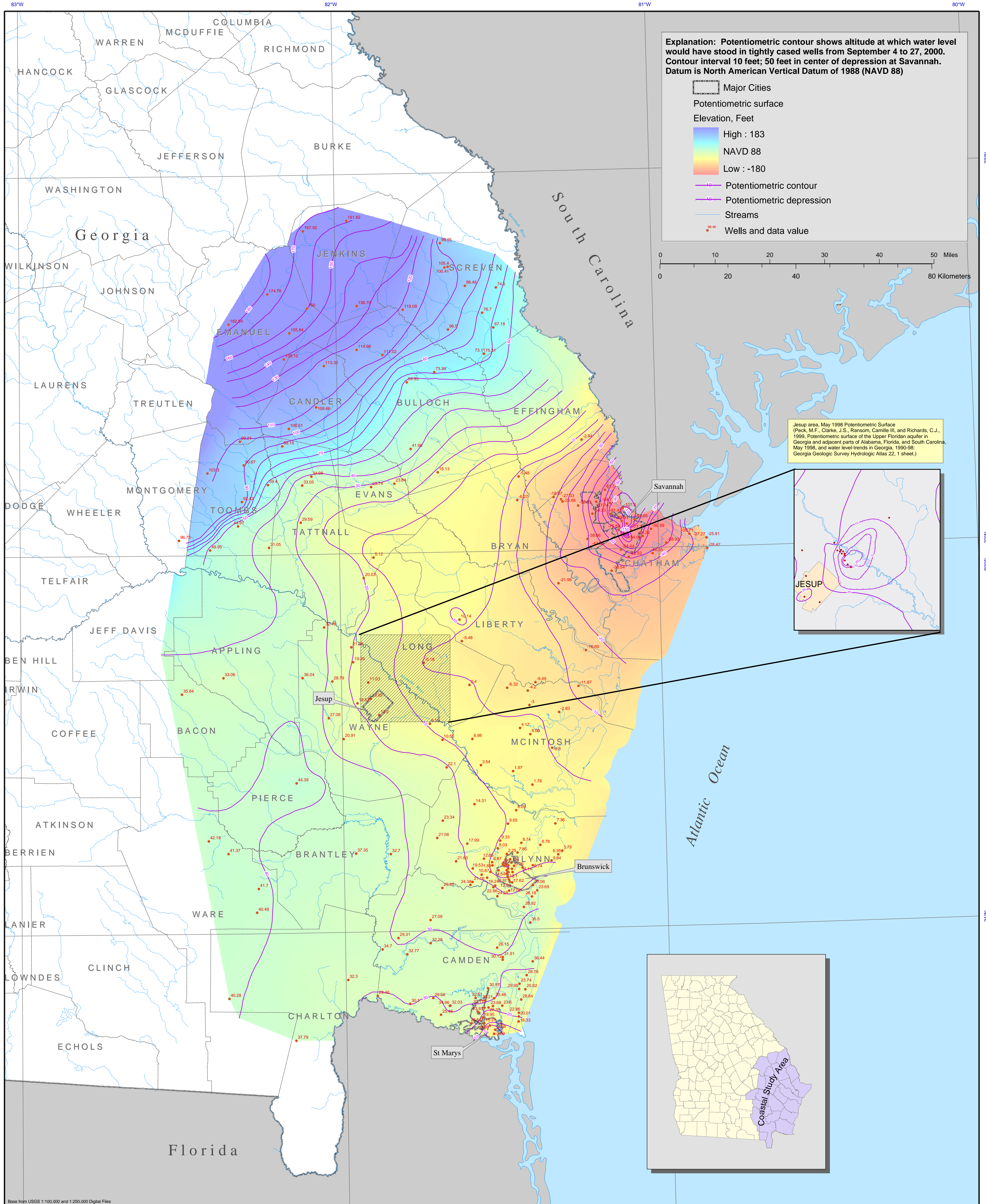
Potentiometric Surface of the Upper Floridan Aquifer in the Coastal Area of Georgia, September 2000
