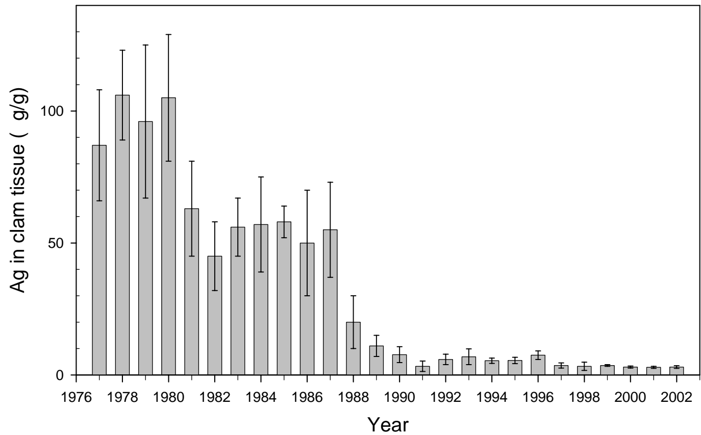
Figure 10. Annual mean concentrations of silver in Macoma balthica at Palo Alto from 1977 through 2002. Error bars are the standard error of the mean (SEM).
