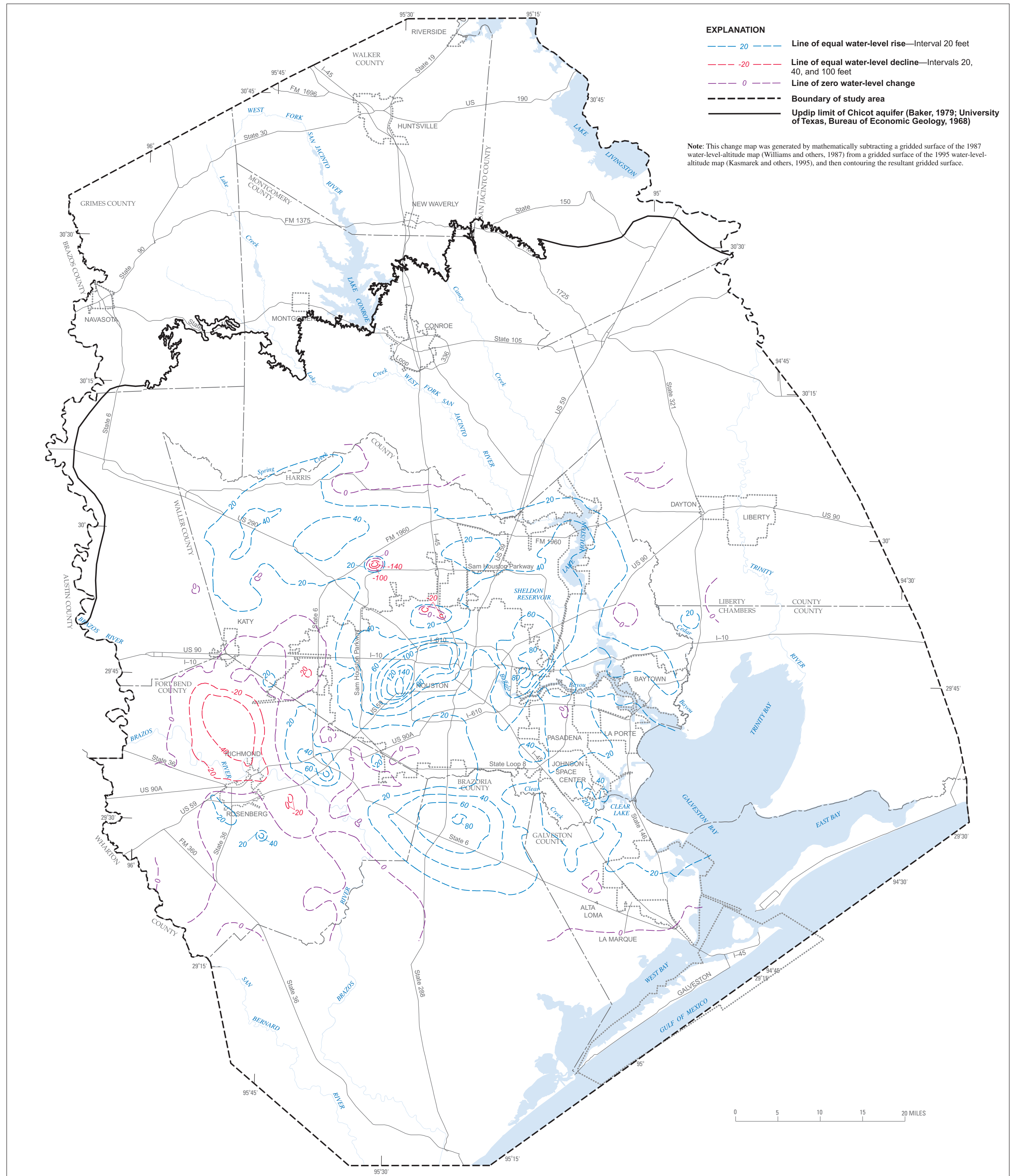
Figure 2. Map showing approximate water-level changes in the Chicot aquifer, Houston-Galveston region, Texas, 1987-95.
