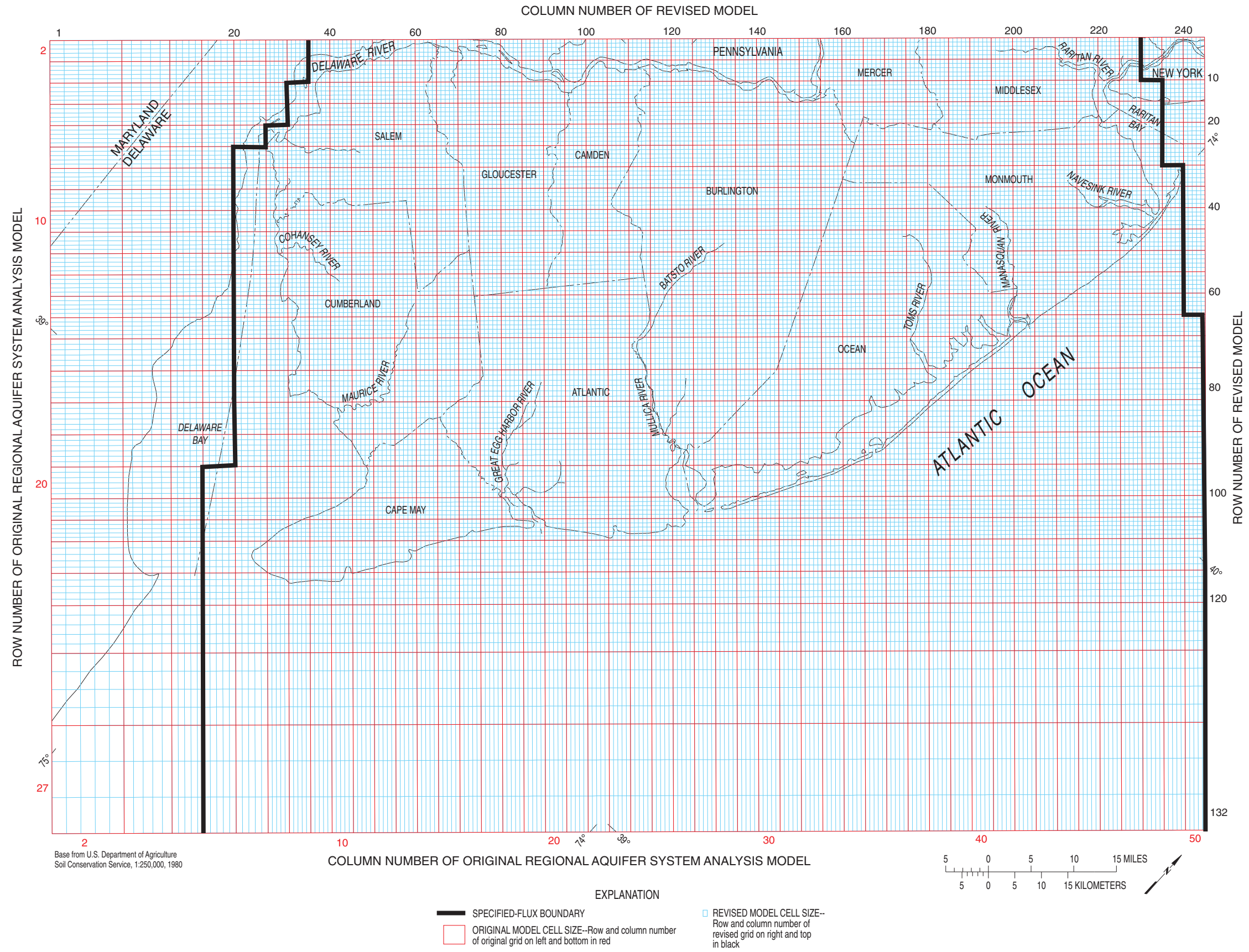
FINITE-DIFFERENCE GRID AND GENERALIZED LATERAL BOUNDARIES OF THE ORIGINAL AND REVISED REGIONAL AQUIFER SYSTEM ANALYSIS MODELS OF THE NEW JERSEY COASTAL PLAIN
