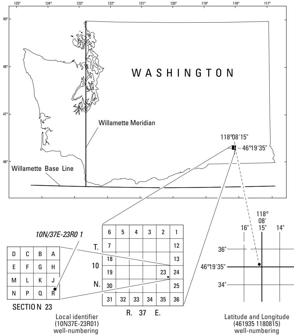
Figure 7. Well-numbering systems used in the State of Washington.
