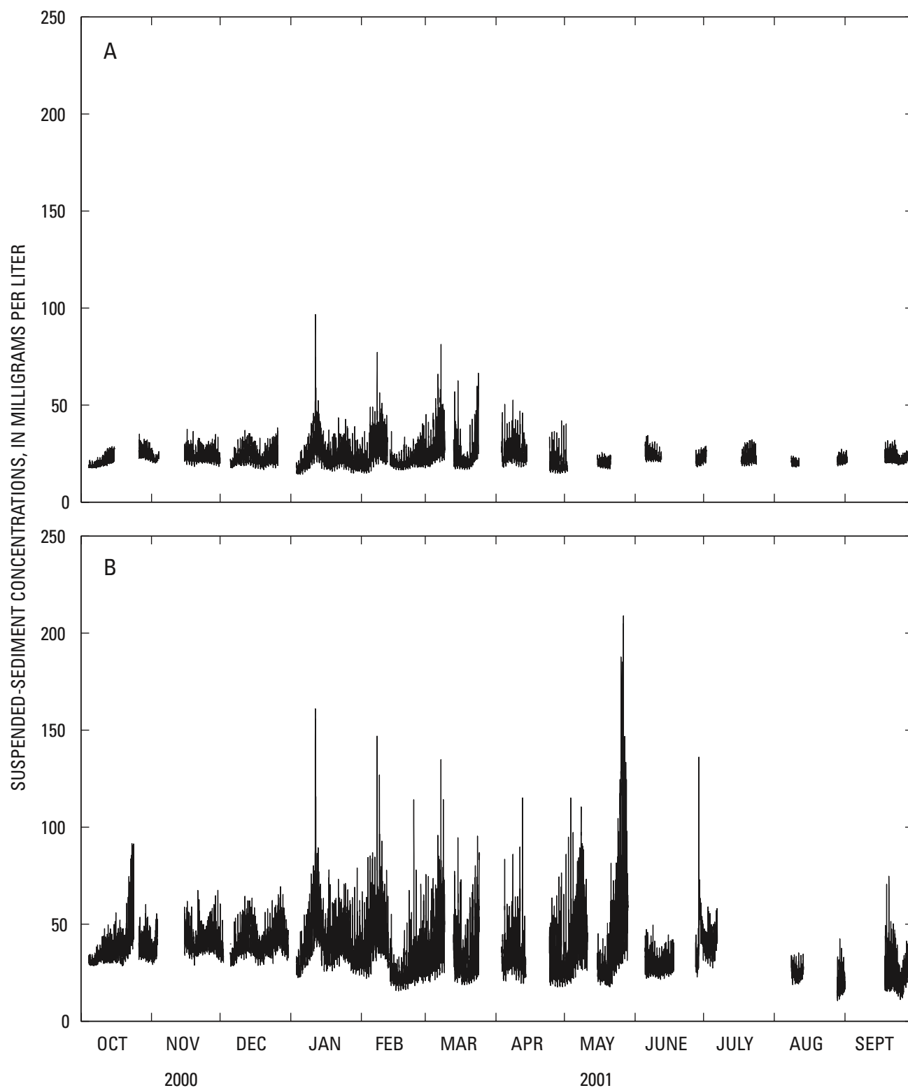
Figure 20. Time series of (A) mid-depth and (B) near-bottom suspended-sediment concentrations calculated from sensor readings at Pier 24, Central San Francisco Bay, California, water year 2001.
